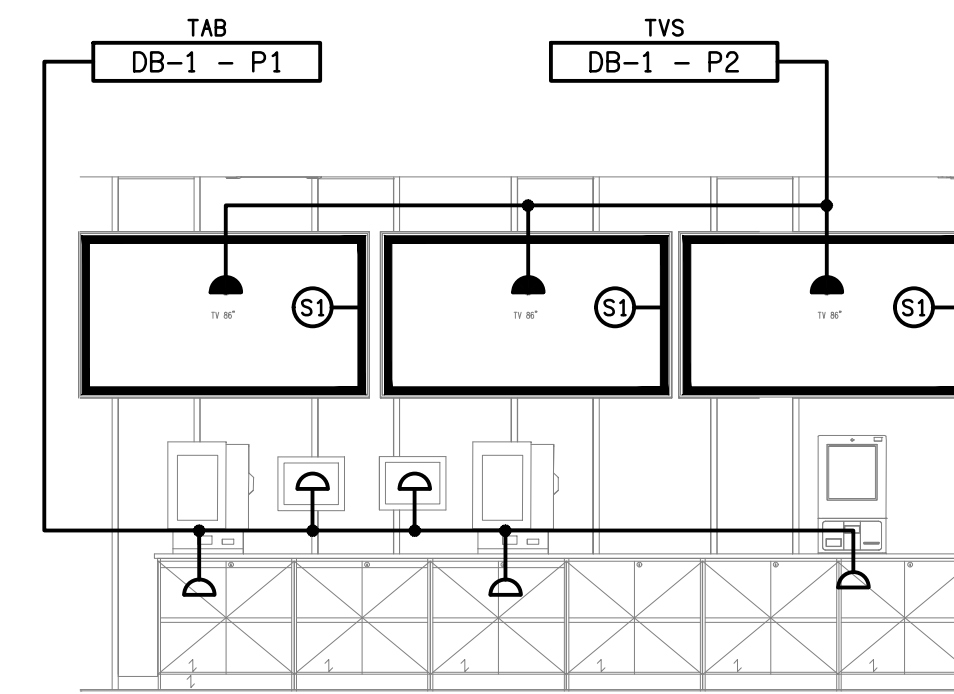
DETAIL A TAB WALL ELEVATION SCALE 1:50
